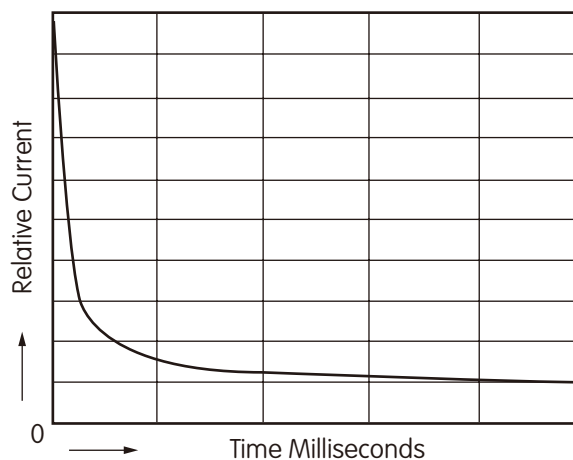
Typical Tungsten Inrush Curve
